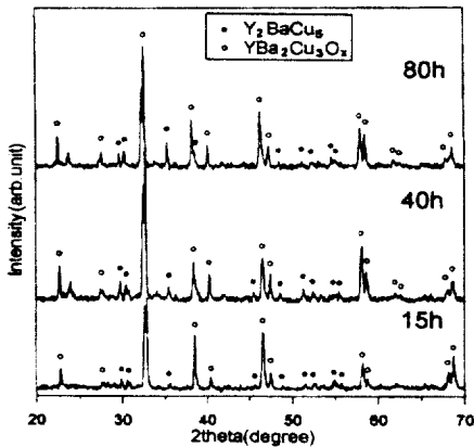
(a) YBa_2Cu_3O_x:Y_2BaCuO_5=1:0.0
