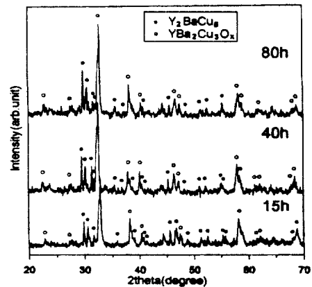
(c) YBa_2Cu_3O_x:Y_2BaCuO_5=1:0.4
