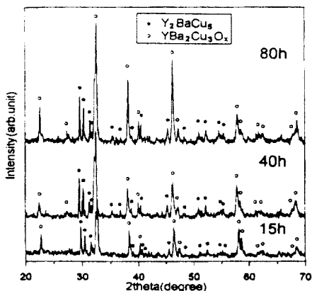
(b) YBa_2Cu_3O_x:Y_2BaCuO_5=1:0.4
