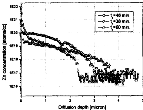
Fig. 3 SIMS profiles for the InP/InGaAs epitaxial structures
