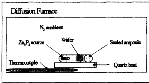
Fig. 2 Schematic diagram of diffusion furnace
