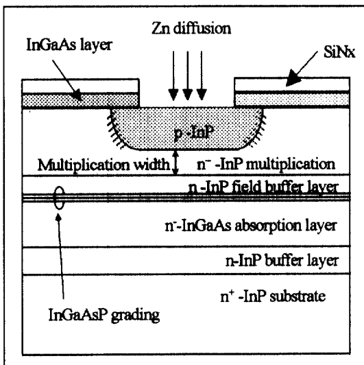
Fig. 1 Schematic diagram of InP/InGaAs test structure
