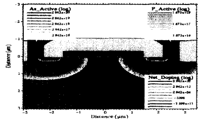
(b) 2-dimensional doping profile
