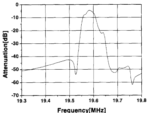
(a) C=0[pF]
