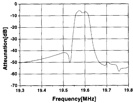
(b) C=15[pF]
