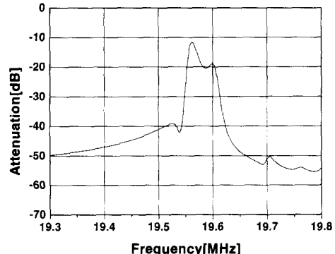
(c) C=100[pF]
