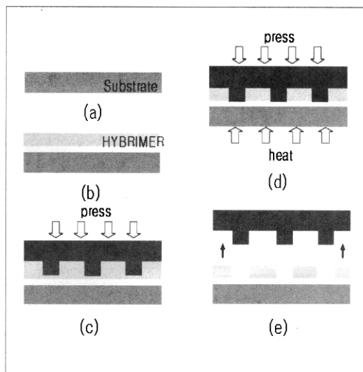
Fig. 1. Fabrication process of a planar waveguide: (a) under-cladding layer formation, (b) core layer formation, (c) first master pressurization, (d) heat and second pressurization, and (e) master separation.
