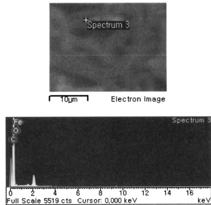
그림 4. 산소 플라즈마 처리된 시편의 EDX 분석. Fig. 4. EDX analysis of carbon nanotubes treated in O 2 plasma. The plasma power and the treatment time was 300 Watt and 30 min, respectively.
