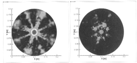
(a) electrons
