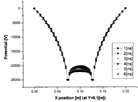
(a) 5.2 cm diam. grid cathode
