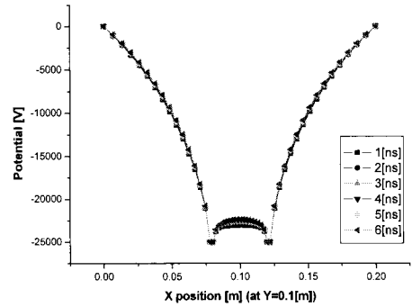
(b) 4.0 cm diam. grid cathode
