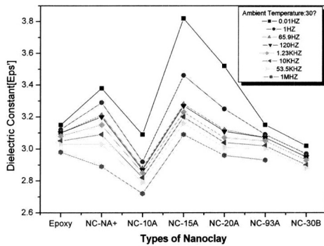
그림 6. Epoxy/organoclay nanocomposites 유전율 특성(Ambient Temp: 30 °C). Fig. 6. Dielectric constant characteristics of epoxy/organoclay nanocomposites(Ambient Temp: 30 °C).
