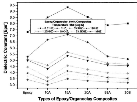
그림 7. Epoxy/organoclay composites 유전율 특성(Ambient Temp: 150 °C). Fig. 7. Dielectric constant characteristics of epoxy/organoclay nanocomposites(Ambient Temp: 150 °C).
