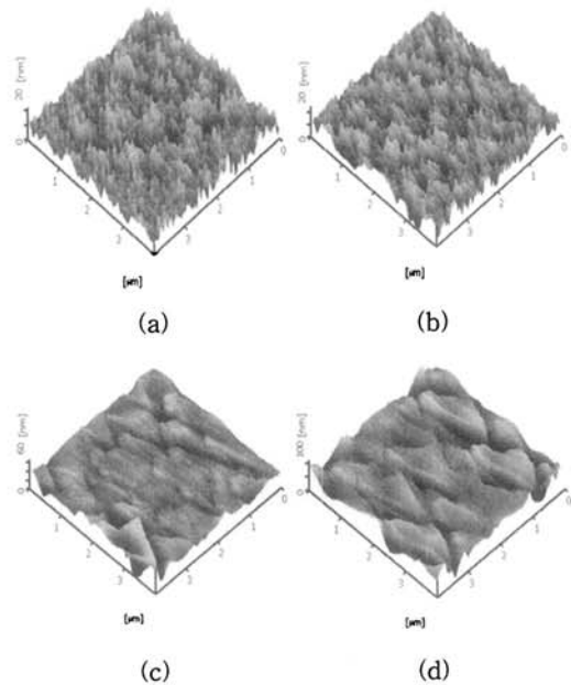
그림 5. (a) 0, (b) 10, (c) 40, (d) 100 sccm으로 각각 도핑된 다결정 3C-SiC 박막의 AFM 이미지. Fig. 5. AFM images of poly 3C-SiC thin films according to (a) 0, (b) 10, (c) 40 and (d) 100 sccm N 2 flow rate, respectively.
