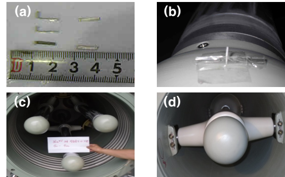
Fig. 6. Photos of metallic defect, and attached inside GIB. (a) Defects (b) Defect on 1 phase GIB (c) Defect on 3 phase end part of GIB (d) Defect on 1 phase end part of GIB
