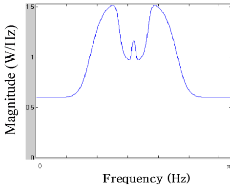
Fig. 1. Modified Fermi filter.
