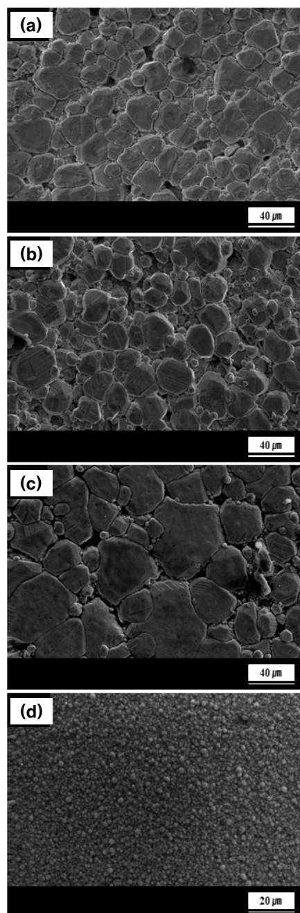
Fig. 6. Surface SEM images of (1-x)\text{BT}-x\text{BNT} ceramics; (a) x=0.01 , (b) x=0.03 , (c) x=0.06 , and (d) x=0.08 .
