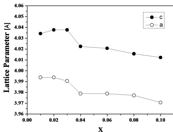
Fig. 5. Variation of lattice parameter of (1-x)\text{BT}-x\text{BNT} ceramics.
