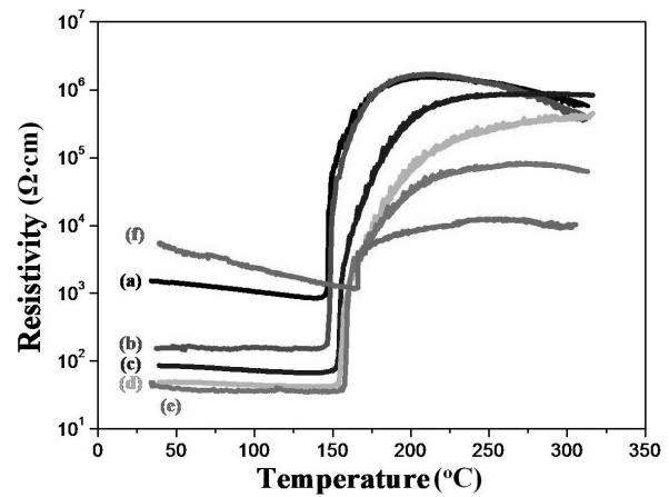
Fig. 7. Temperature dependence of resistivity of the (1-x)BT-xBNT PTCT ceramics; (a) x=0.01, (b) x=0.02, (c) x=0.03, (d) x=0.04, (e) x=0.06, and (f) x=0.08.
