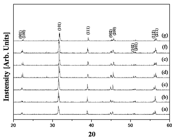
Fig. 4. X-ray diffraction patterns of (1-x)\text{BT}-x\text{BNT} ceramics; (a) x=0.01 , (b) x=0.02 , (c) x=0.03 , (d) x=0.04 , (e) x=0.06 , (f) x=0.08 , and (g) x=0.10 .
