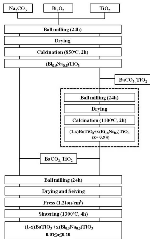
Fig. 1. The flow chart of (1-x)\text{BT}-x\text{BNT} ( 0.01 \leq x \leq 0.10 ) PTCT thermistor by modified synthesis process.
