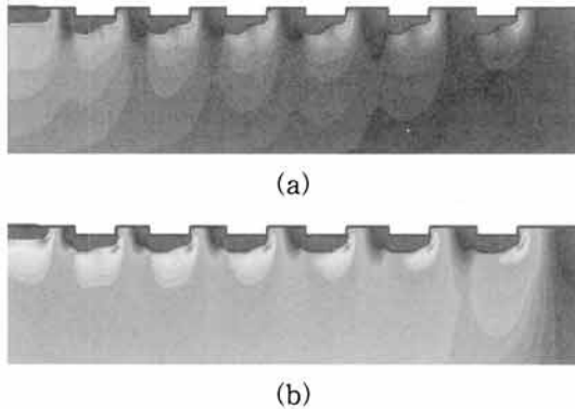
Fig. 5. (a) Electric field of the trench etched field ring with dual ion-implantation for 15 \mu\text{m} window width, (b) Electric field of the trench etched field ring with dual ion-implantation for 15/18/21/24/27/30 \mu\text{m} window width.
