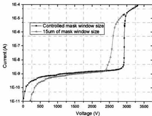
Fig. 6. I-V curve of trench etched field ring with dual ion-implantation applied 15 \mu\text{m} window width and 15/18/21/24/27/30 \mu\text{m} controlled window width.
