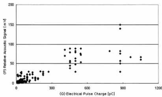
(b) Output response of AE sensor with non-coupled vibration mode
