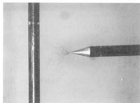
Fig. 5. Electric tree generation of XLPE sheets.
