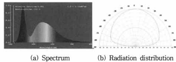
Fig. 4. Optic properties of single LED.
