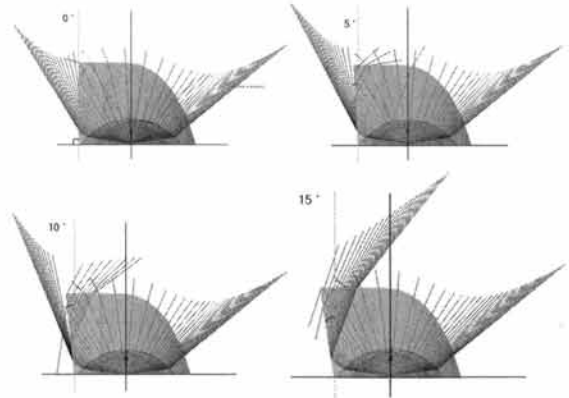
Fig. 6. Ray properties according to change incline angle of the second surface.
