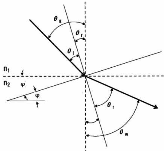
Fig. 1. Determination of refractor segments.
