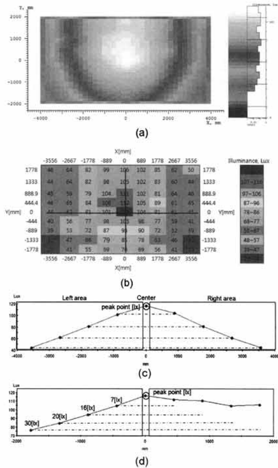
Fig. 10. Illuminance distribution properties according to installation height (installation height 4 m, applied area 8 m × 4 m).
