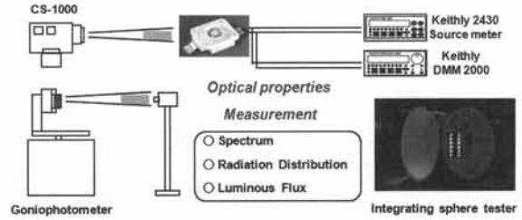
Fig. 2. Experimental set up of single LED.
