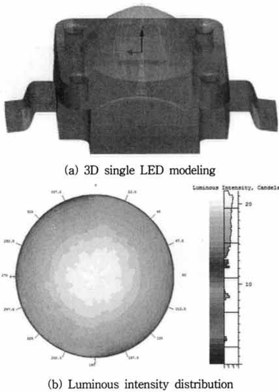
Fig. 5. Designed 3D modeling and optic properties.
