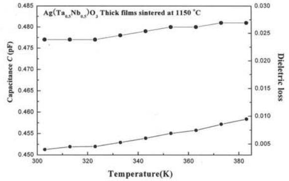
Fig. 3. Temperature dependent capacitance and dielectric loss of ATN thick film.
