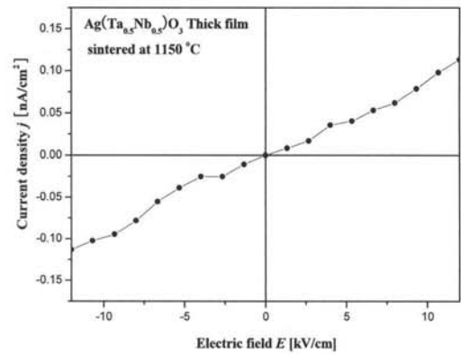
Fig. 4. The current voltage characteristics of ATN thick film.
