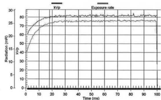
Fig. 4. The change to X-ray exposure time of dual voltage rectification method.
