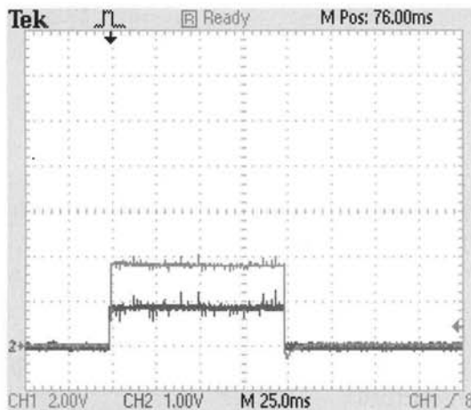
Fig. 6. Ripple of dual voltage rectification method.
