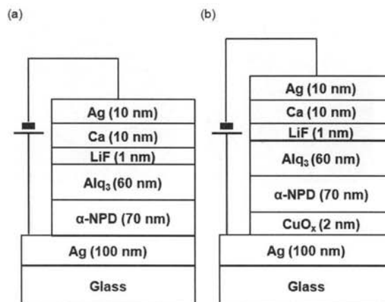
Fig. 1. Device structure of (a) "Ag" and (b) "Ag/ \text{CuO}_x ".
