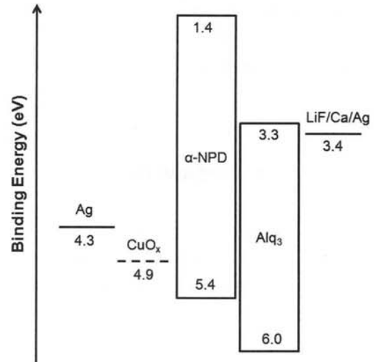
Fig. 4. Energy level diagrams of the individual device components. The change of work function of the Ag and CuO x were determined using a synchrotron radiation photoemission spectroscopy. The energy levels for other components are taken from the literature.
