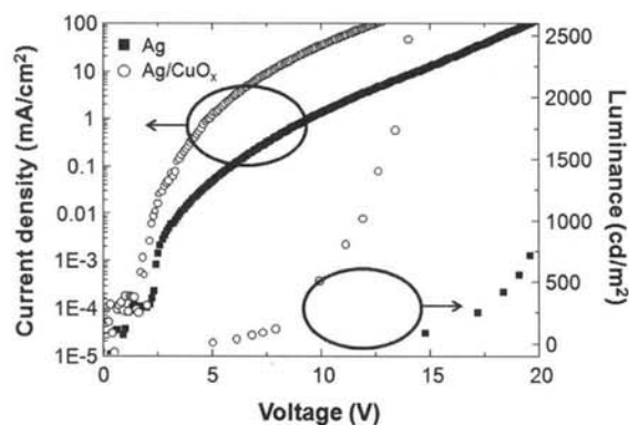
Fig. 2. Current density-voltage (log plot) and luminance-voltage (linear plot) characteristics of TEOLEDs with "Ag" and "Ag/ \text{CuO}_x " anodes.
