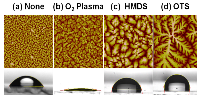
Fig. 5. AFM image ( 5\ \mu\text{m} \times 5\ \mu\text{m} ) of the pentacene films deposited on the cross-linked PVP gate dielectrics treated by various method: (a) no treat, (b) \text{O}_2 plasma, (c) HMDS, (d) OTS. In each condition, the water contact angle of PVP surface is 49^\circ , 6^\circ , 75^\circ , and 102^\circ , respectively.
