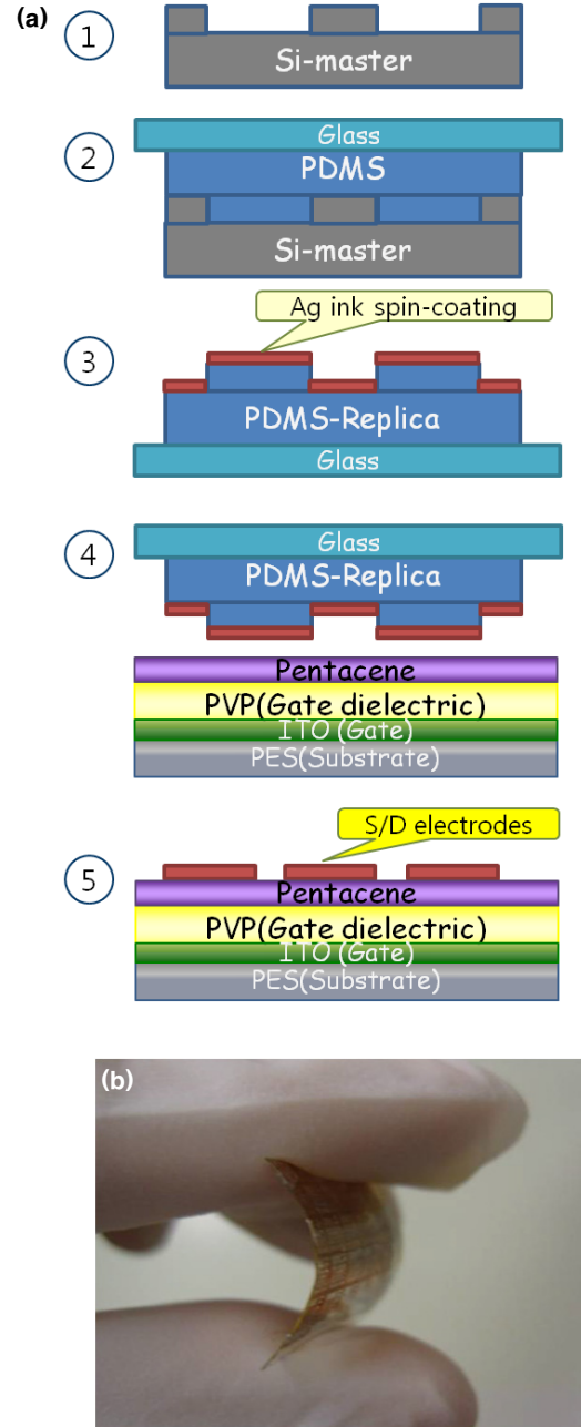
Fig. 3. (a) The schematic diagram of the S/D formation flow using micro contact printing method. (b) Fabricated OTFT on flexible substrate. Here, the channel length is 1 \mu\text{m} and width is 100 \mu\text{m} .
