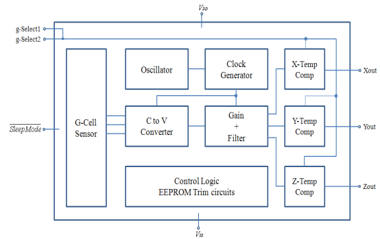
Fig. 1. Block diagram of the 3 axis accelerometer sensor.
