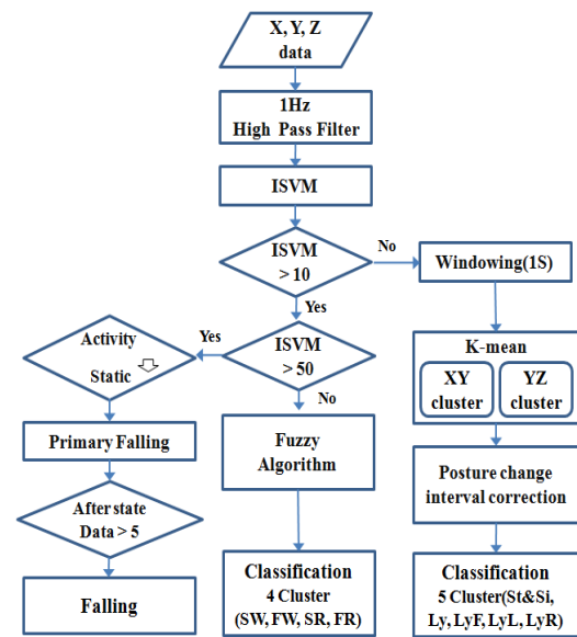
Fig. 3. Flow chart of the activity classification algorithm.
