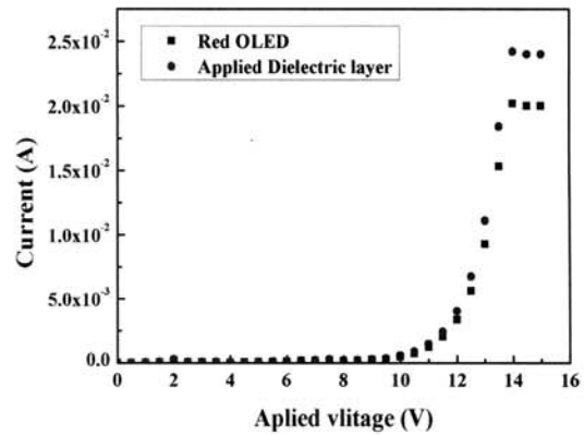
Fig. 5. Current-voltage characteristics of red organic emitting device with anti-refractive layer.
