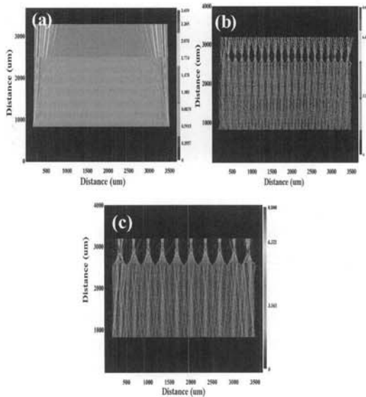
Fig. 7. FDTD simulation result of micro lens. (a) no lens, (b) 5 um lens, (c) 10 um lens.
