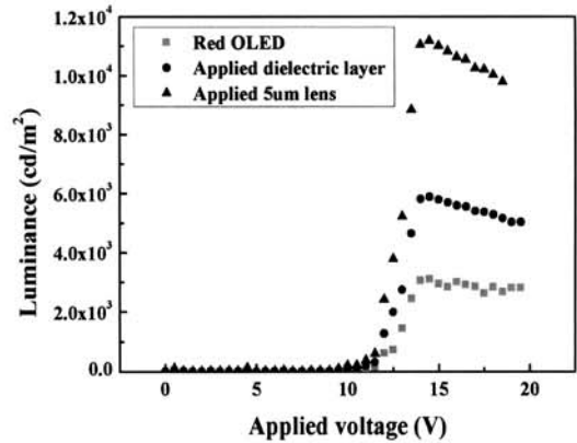
Fig. 9. Voltage-luminance characteristics of red organic emitting device with 5um micro lens.
