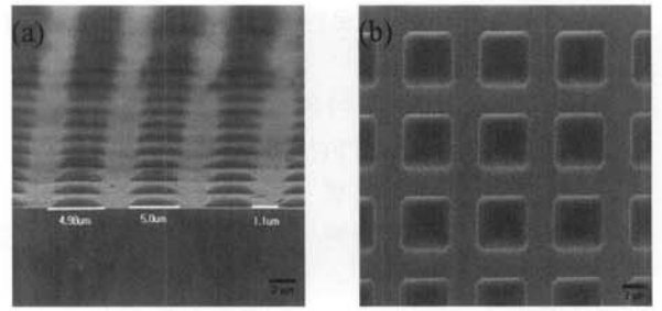
Fig. 8. SEM image of micro lens. (a) cross section image micro lens, (b) surface section image micro lens.
