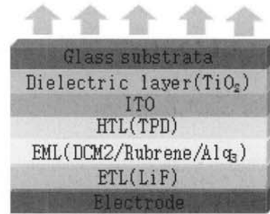
Fig. 2. Red organic device applied anti-refractive layer.
