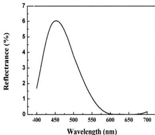
Fig. 4. Simulation result of organic material/ITO/TiO 2 /glass structure.
