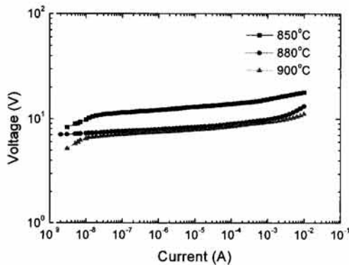
Fig. 3. I-V characteristics of ZnO chip varistors with sintering temperatures.
