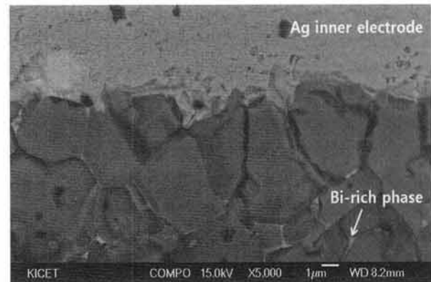
Fig. 2. Microstructure of ZnO chip varistor sintered at 900°C.
