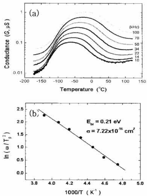
Fig. 4. (a) admittance spectra at 10~100 kHz for ZnO chip varistor sintered at 900°C, (b) ln(ω/T p 2 ) vs. 1,000/T.
