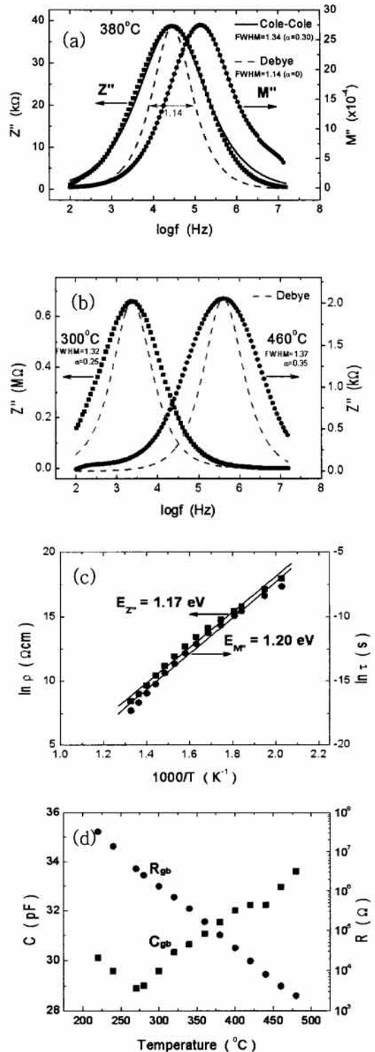
Fig. 5. Impedance and modulus spectroscopy of ZnO chip varistor sintered at 900^\circ\text{C} . (a) Z'' -, M'' -logf ( 380^\circ\text{C} ), (b) Z'' -logf ( 300 and 460^\circ\text{C} ), (c) \ln \rho and \ln \tau vs. 1,000/T plot, (d) resistance ( R_{gb} ) and capacitance ( C_{gb} ) with temperature.
