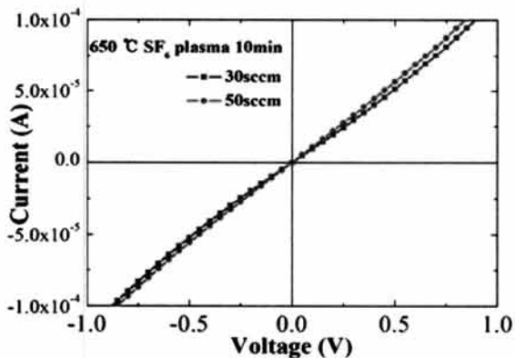
Fig. 4. Typical I-V characteristics measured from F-doped ITO contacts under different gas rates.
