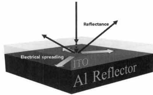
Fig. 1. Schematic diagram of ITO/Al based reflector.
