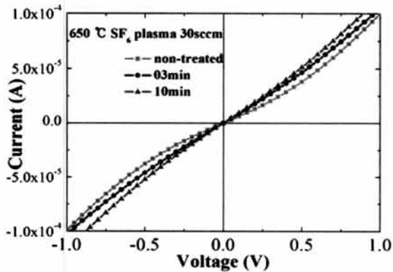
Fig. 3. Typical I-V characteristics measured from F-doped ITO contacts under different times.
