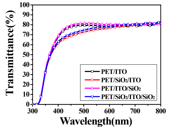
Fig. 7. Optical properties of the ITO thin films by an insertion of SiO 2 thin films.
