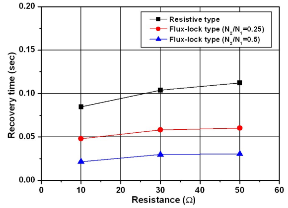
Fig. 8. Recovery characteristics of the resistive type and the flux-lock type SFCL according to turn's ratio.
