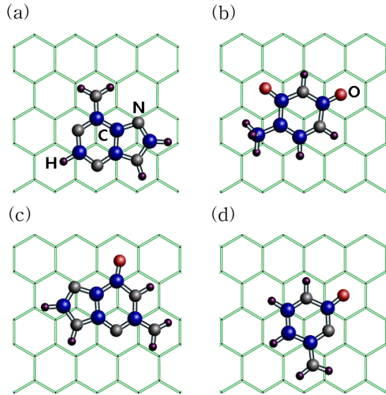
Fig. 1. Atomic structures of (a) adenine, (b) thymine, (c) guanine, and (d) cytosine adsorbed on graphene.
