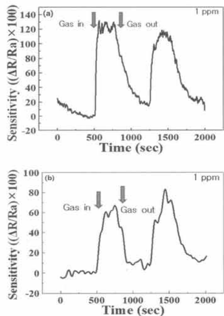
Fig. 5. The sensitivity of ethanol gas sensor for 1 ppm at 300℃ of (a) pure ZnO and (b) 1GZO.
