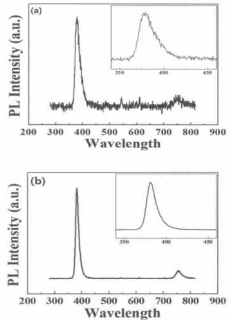
Fig. 4. Photoluminescence data of (a) pure ZnO, and (b) 1GZO.
