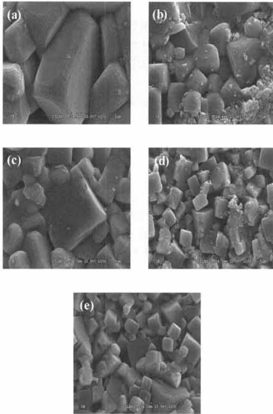
Fig. 2. Microstructure of specimens as a function of Sb substitution. (a)-0mol%Sb, (b)-2mol%Sb, (c)-4mol%Sb, (d)-6mol%Sb, and (e)-8mol%Sb.
