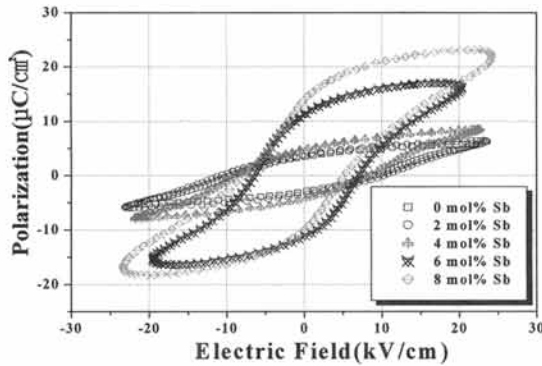
Fig. 9. P - E hysteresis loops of specimens as a function of Sb substitution.
