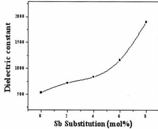
Fig. 7. Dielectric constant of specimens as a function of Sb substitution.
