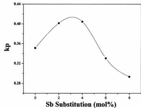
Fig. 4. Electromechanical coupling coefficient(kp) of specimens as a function of Sb substitution.
