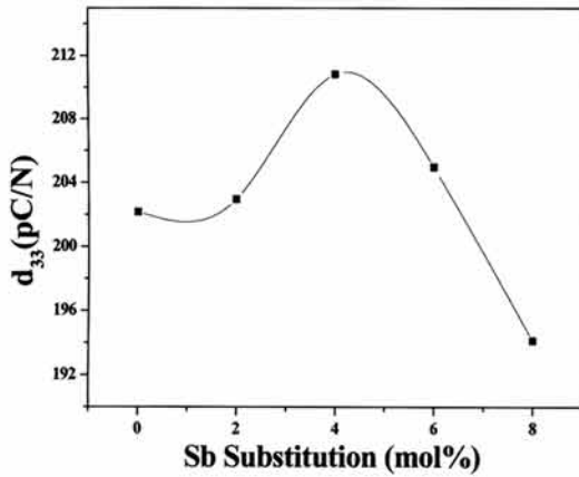
Fig. 5. Piezoelectric coefficient( d_{33} ) of specimens as a function of Sb substitution.
