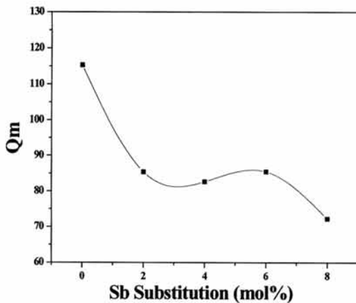
Fig. 6. Electromechanical quality factor( Q_m ) of specimens as a function of Sb substitution.
