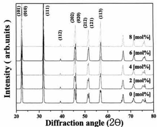
Fig. 1. X-ray diffraction patterns of specimens as a function of Sb substitution.
