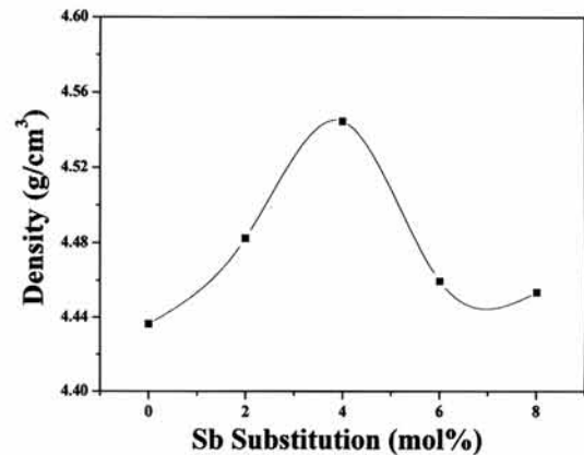
Fig. 3. Density of specimens as a function of Sb substitution.
