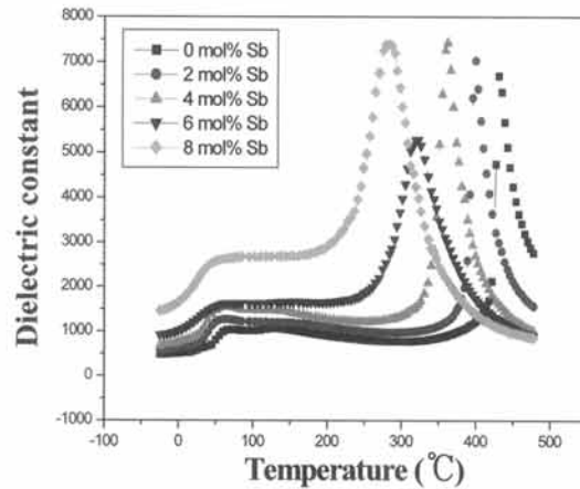
Fig. 8. Temperature dependence of dielectric constant of specimens as a function of Sb substitution.
