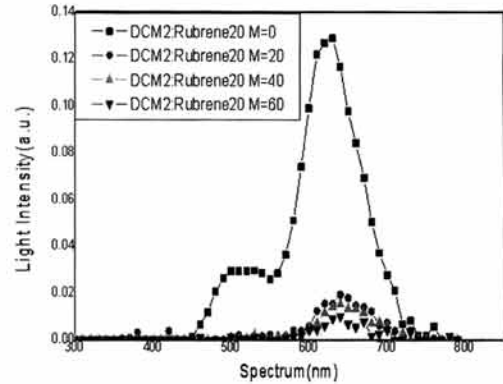
Fig. 4. Spectrum of red OLED.
