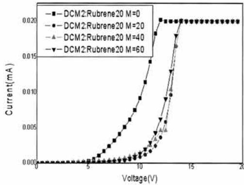
Fig. 2. Voltage-current characteristics of red OLED.
