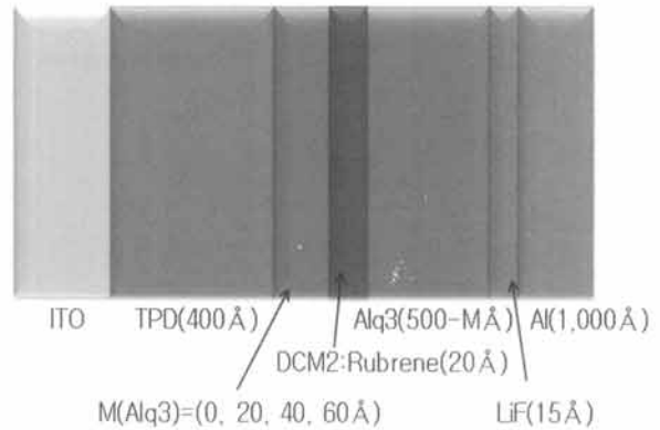
Fig. 1. Structure of red organic light emitting diode.
