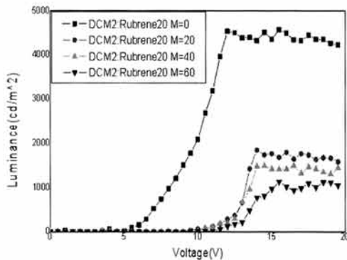
Fig. 3. Voltage-luminance characteristics of red OLED.
