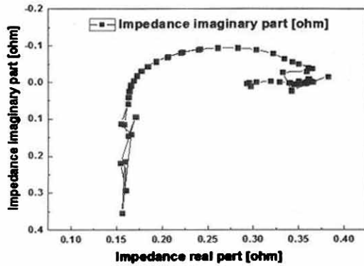
Fig. 8. Solar cell electrical characteristics of frequency variation at 121.9 lux.
