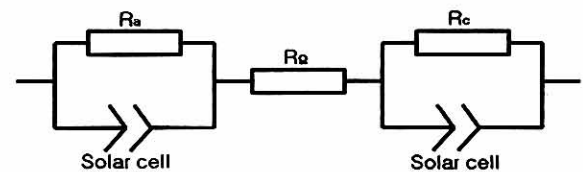
Fig. 4. Internal equivalent circuit of solar cell.
