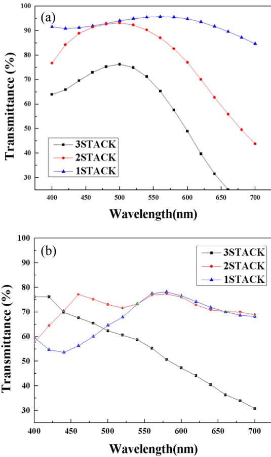
Fig. 1. Simulation results with different stacking sequence in: (a) TiO 2 /Ag/TiO 2 and (b) TiO 2 /Si 3 N 4 /Ag/Si 3 N 4 /TiO 2 .
