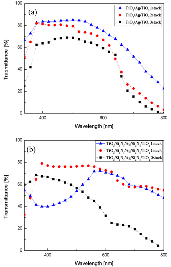
Fig. 2. Transmittance of (a) TiO 2 /Ag/TiO 2 , (b) TiO 2 /Si 3 N 4 /Ag/Si 3 N 4 /TiO 2 multi-layered structure with increasing the stacking times in visible range.
