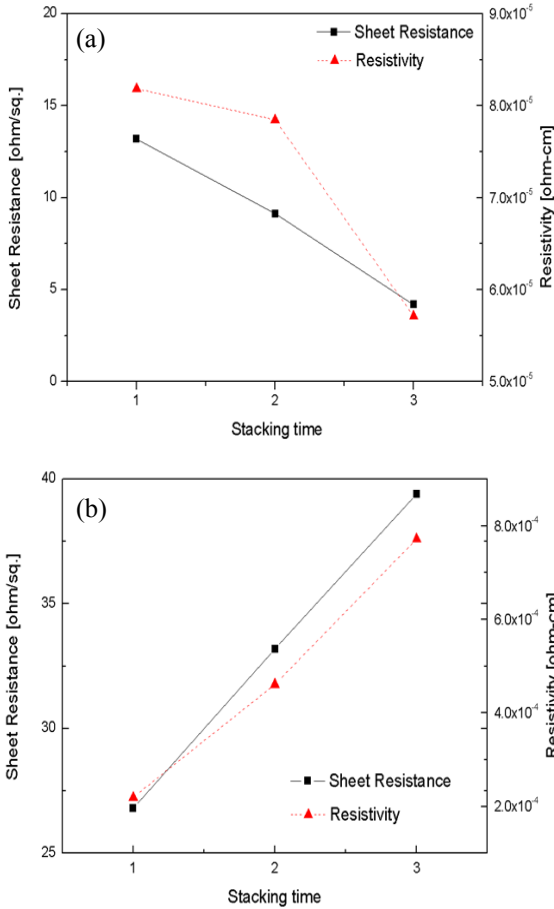
Fig. 3. The surface resistance and resistivity variation with increase of stacking times; (a)TiO 2 /Ag/TiO 2 layer and (b)TiO 2 /Si 3 N 4 /Ag/Si 3 N 4 /TiO 2 layer.
