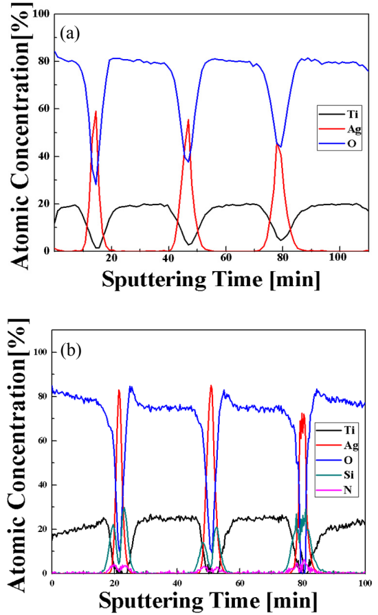
Fig. 4. AES depth profile of multi-layered structure; (a) TiO 2 /Ag/TiO 2 layer and (b) TiO 2 /Si 3 N 4 /Ag/Si 3 N 4 /TiO 2 layer.
