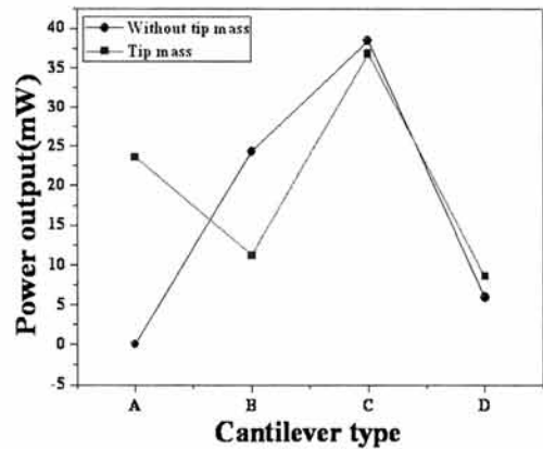
Fig. 7. Output power harvested from the various kinds of SPCS with optimized tip mass and without tip mass for 15s under a base acceleration magnitude of 0.5 G.
