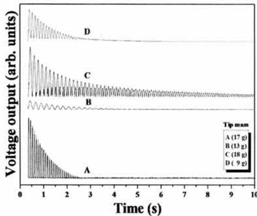
Fig. 5. Peak voltage response for the various kinds of SPCS with each tip mass under a base acceleration magnitude of 0.5 G.
