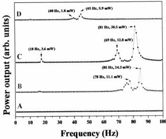
Fig. 3. Variations of the output power as a function of applied frequency for the various kinds of SPCS without tip mass.
