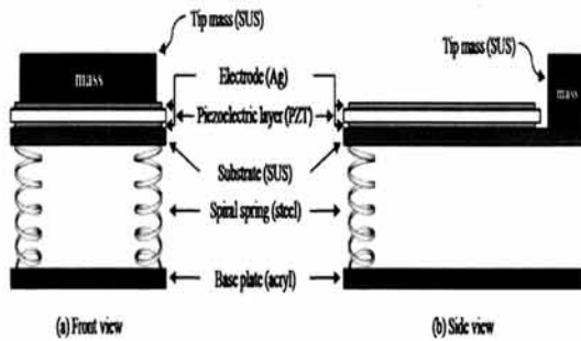
Fig. 2. Schematic diagram of the proposed piezoelectric cantilever spring structure (SPCS); (a) front view and (b) side view.
