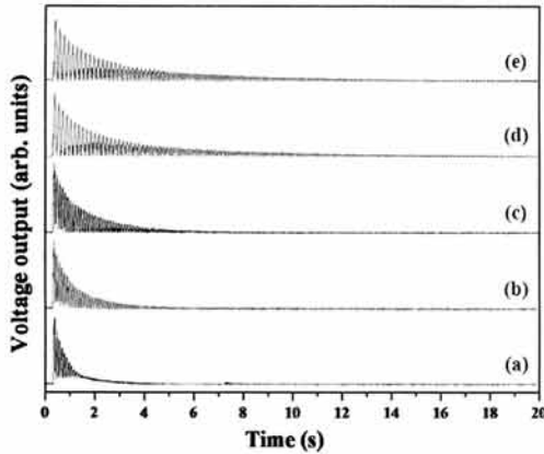
Fig. 4. Voltage response for the C type SPCS as a function of tip mass under base acceleration of 0.5 G (a) 6 g, (b) 7 g, (c) 8 g, (d) 17 g, and (e) 18 g.
