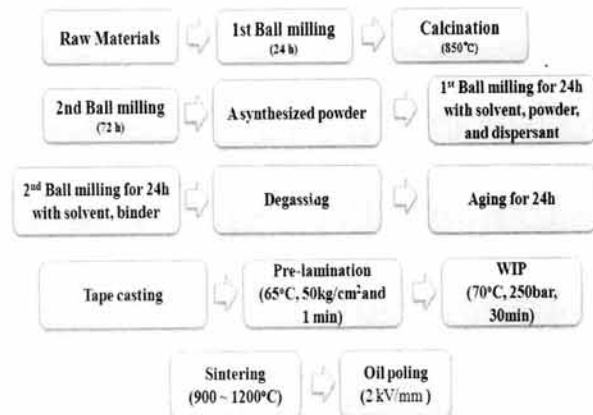
Fig. 1. 0.72PZT-0.28PZNN piezo thick film process and production method.
