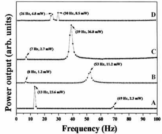
Fig. 6. Variations of the output power as a function of applied frequency for the various kinds of piezoelectric cantilever generators with each tip mass.
