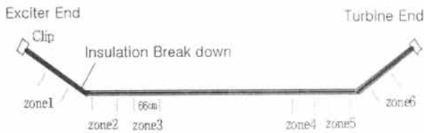
Fig. 4. Structure of B generator stator windings.
