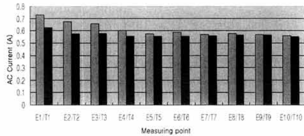
Fig. 8. Comparison of AC leakage current in A generator stator windings.
