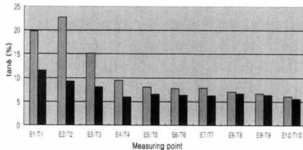
Fig. 6. Comparison of dissipation factor in A generator stator windings.
