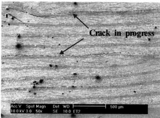
Fig. 12. SEM micrograph of zone 6 stator winding.
