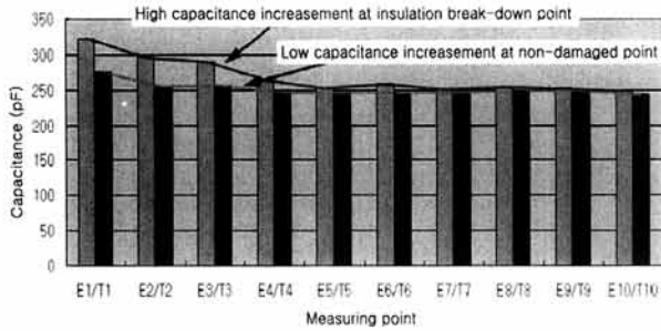
Fig. 7. Comparison of capacitance in A generator stator windings.
