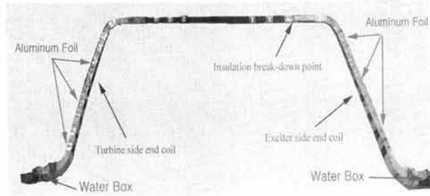
Fig. 3. Structure of A generator stator windings.
