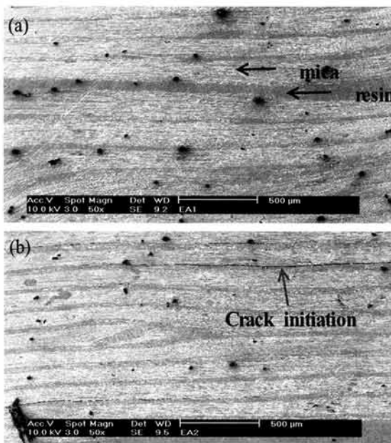
Fig. 9. SEM micrographs of zone 1 stator winding. (a) water box, (b) ground fault.
