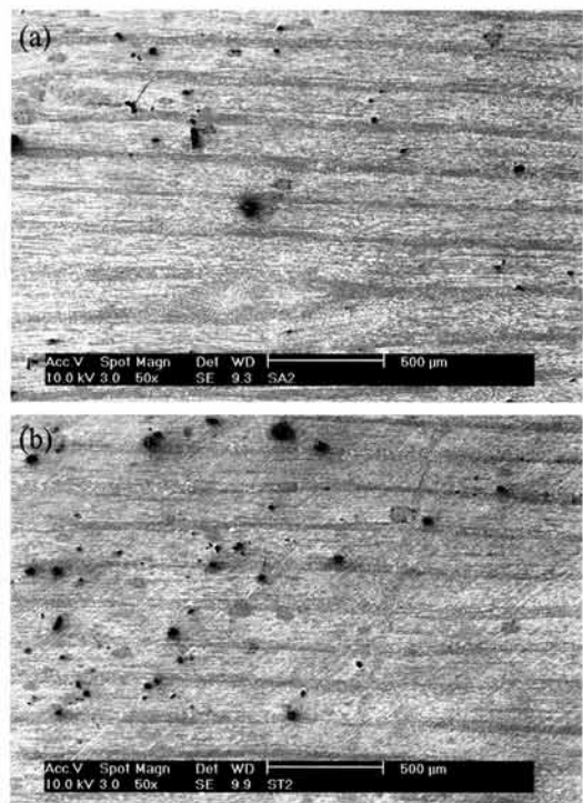
Fig. 11. SEM micrographs of zone 4 and zone 5 stator windings. (a) zone 4, (b) zone 5.
