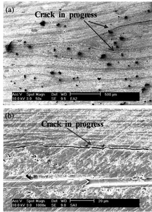
Fig. 10. SEM micrographs of zone 2 stator winding. (a) magnification: 50x, (b) magnification: 1,000x.
