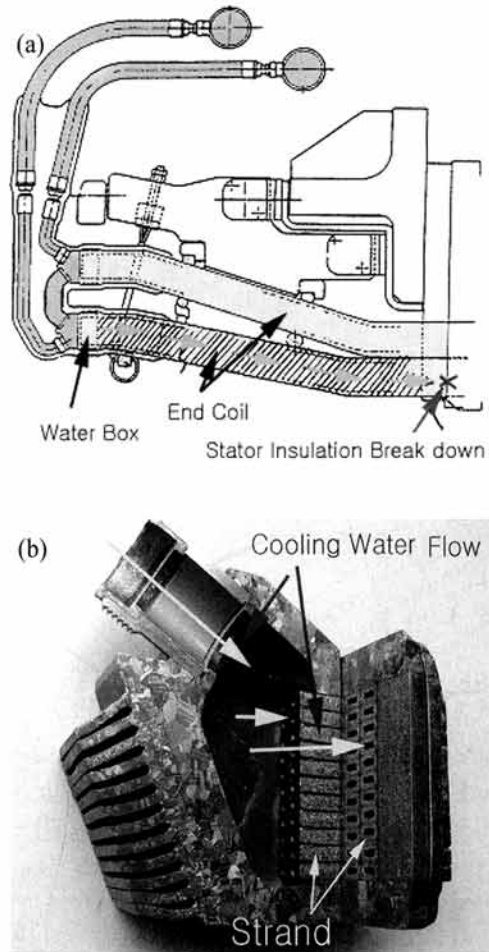
Fig. 2. Water absorption of generator stator windings and water box structure. (a) water absorption, (b) water box structure.
