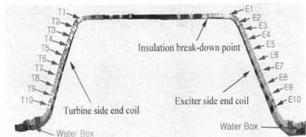
Fig. 5. Measurement position of A generator stator windings.
