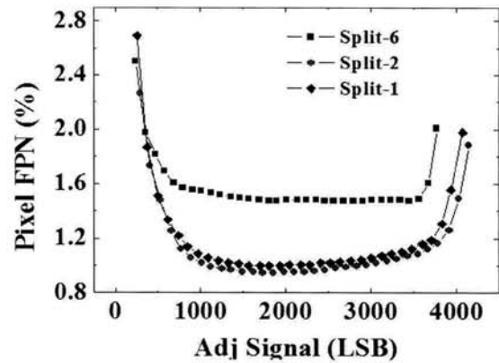
Fig. 4. Pixel FPN result due to microlens focusing.
