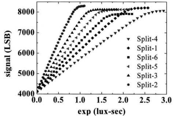
Fig. 3. Green response curve with respect to splits.
