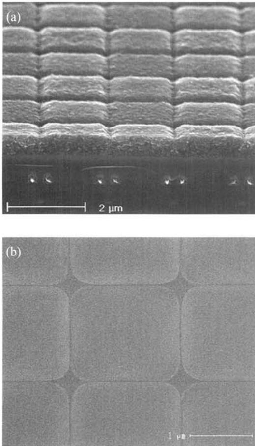
Fig. 1. (a) SEM pictures of cross-section just after the color filter step and (b) TOP view after the completion of full process.
