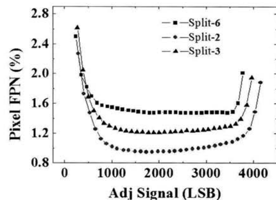
Fig. 5. Pixel FPN result due to the color pattern.
