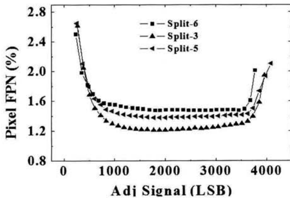
Fig. 6. Pixel FPN result with split of color pattern.
