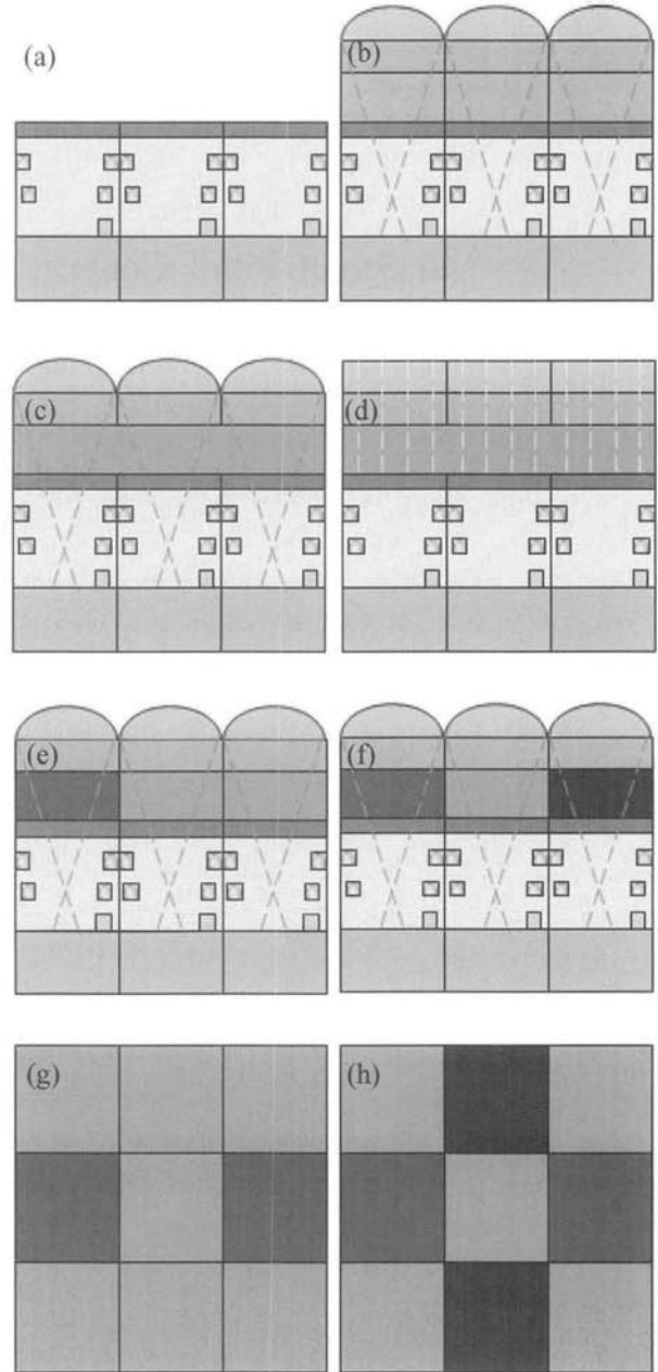
Fig. 2. Split conditions for experiments. (a) split-1 (BW-wafer), (b) split-2(BW+OCL+ML), (c) split-3 (green+OCL+ML), (d) split-4(G+OCL+MLcoat), (e) split-5(R/G+OCL+ML), (f) split-6 (R/G/B+OCL+ML), (g) top view of split-5, and (h) top view of split-6.
