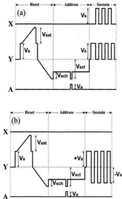
Fig. 4. (a) Modified driving waveform for open dielectric structure and (b) low cost driving waveform.
