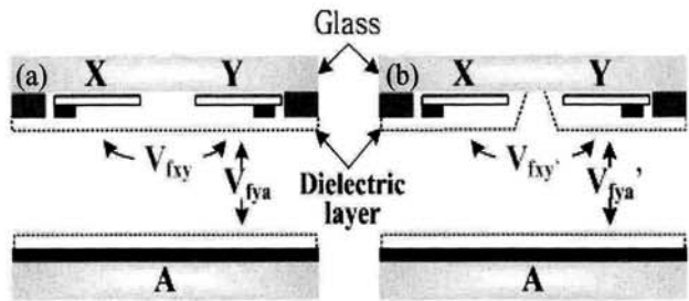
Fig. 1. Schematic diagram of conventional (a) and open dielectric structure (b) of 42 inch AC PDP.
