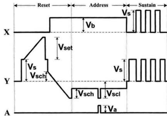
Fig. 2. Conventional driving waveform to applying three electrodes during reset, address, sustain periods.
