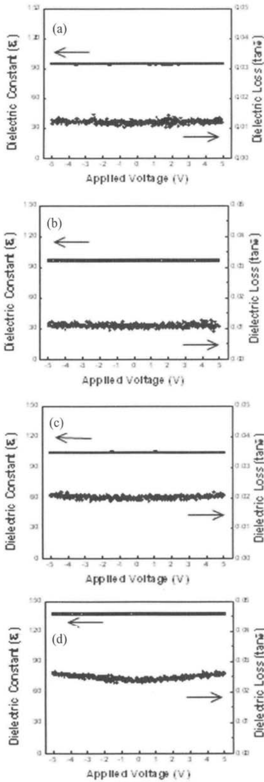
Fig. 2. Voltage dependence of dielectric constant and loss of SBNO thin film with RTA. (a) 650°C, (b) 700°C, (c) 750°C, (d) 800°C.
