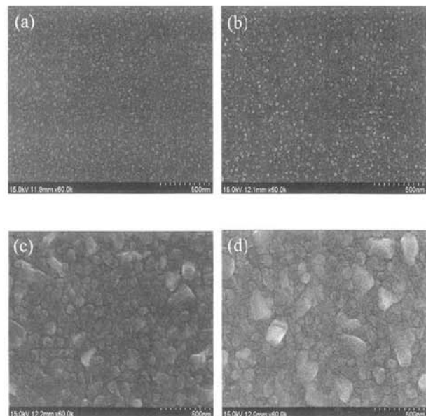
Fig. 1. SEM images of SBNO thin films with RTA. (a) 650^\circ\text{C} , (b) 700^\circ\text{C} , (c) 750^\circ\text{C} , (d) 800^\circ\text{C} .
