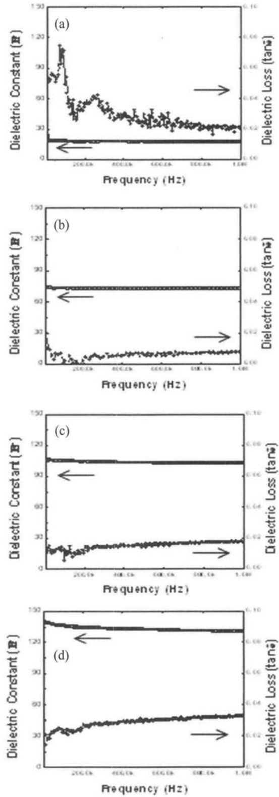
Fig. 3. Frequency dependences of dielectric constant and loss of SBNO thin film with RTA. (a) 650°C, (b) 700°C, (c) 750°C, (d) 800°C.
