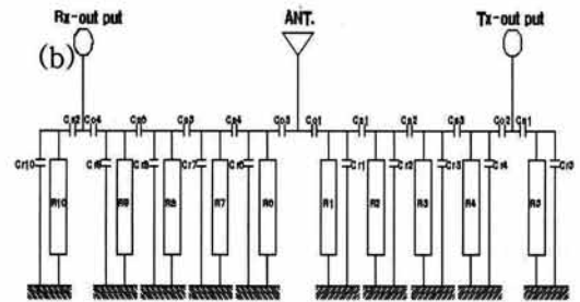
Fig. 2. The circuit of ceramic mono-block BPF and duplexer. (a) The circuit of ceramic mono-block BPF, (b) the circuit of ceramic mono-block duplexer.
