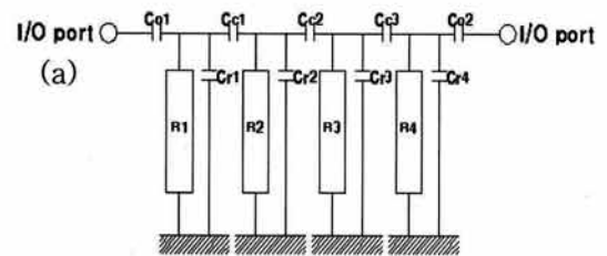
Fig. 1. The inner circuit of ceramic resonator.
