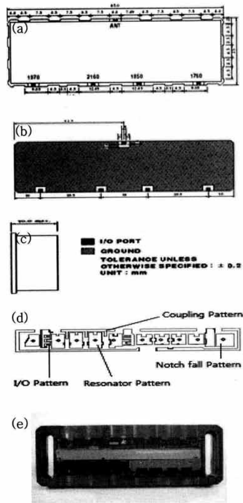
Fig. 3. Four channel multiplexer with common Port of ANT, (a) top view, (b) bottom view, (c) side view, (d) top pattern of W-CDMA duplexer, (e) fabricated four channel multiplexer.
