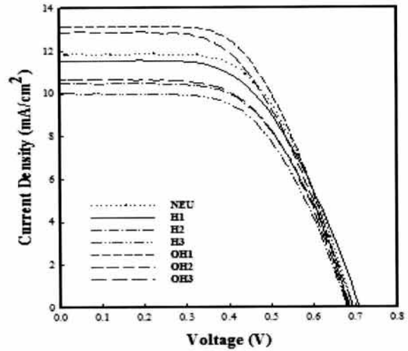
Fig. 4. I-V curve of the DSSC prepared by using NEU, H1, H2, H3, OH1, OH2 and OH3.
