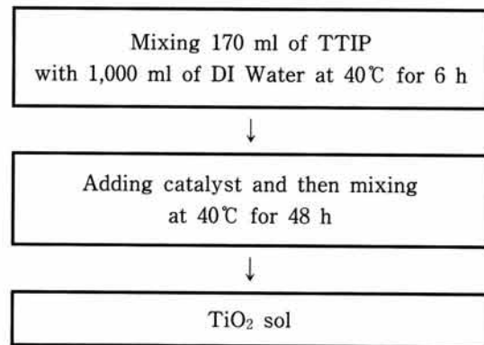
Fig. 1. Flow chart of preparation of TiO 2 sol by sol-gel method.
