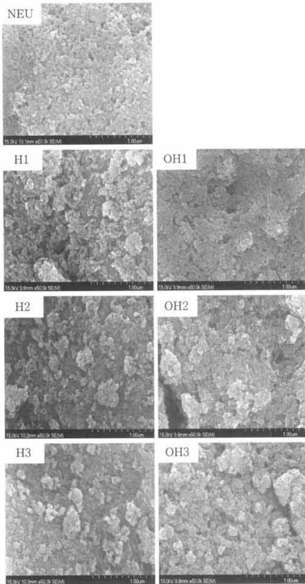
Fig. 3. FE-SEM images of surface morphology of TiO 2 thin films prepared by using NEU, H1, H2, H3, OH1, OH2 and OH3.
