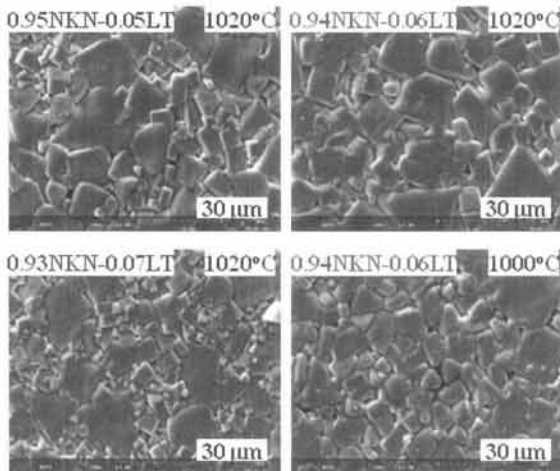
Fig. 3. SEM images of (1-x)NKN-xLT (0.04 ≤ x ≤ 0.07) calcined at 900°C for 4 h and sintered at 1,020°C for 4 h.
