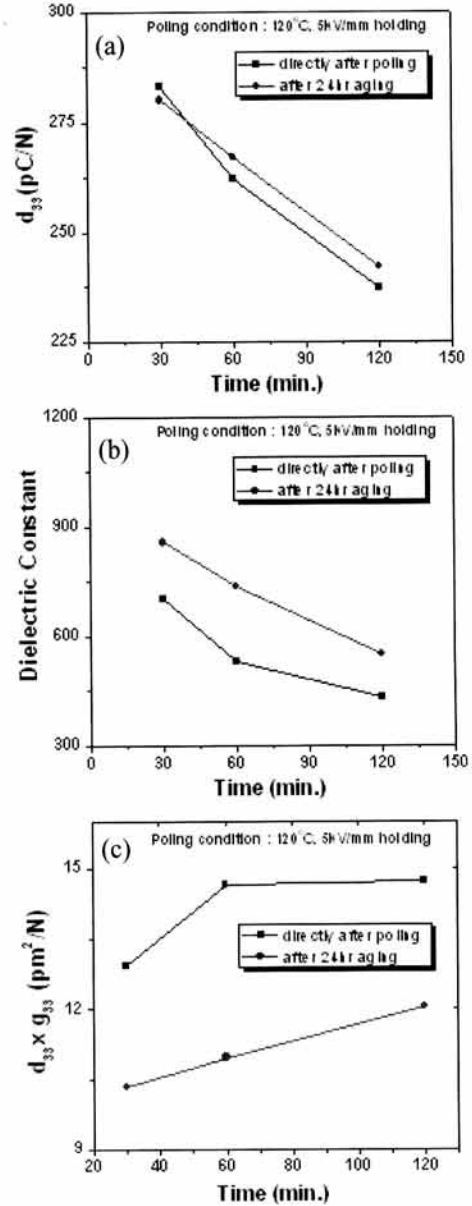
Fig. 15. (a) d_{33} , (b) \epsilon_{33}^T/\epsilon_0 and (c) d_{33} \times g_{33} of (NKN)N 0.990 T 0.010 with changing poling time.
