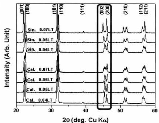
Fig. 1. XRD patterns of (1-x)\text{NKN}-x\text{LT} ( 0.04 \leq x \leq 0.07 ) calcined at 900^\circ\text{C} for 4 h and sintered at 1,020^\circ\text{C} for 4 h.
