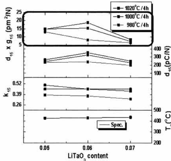
Fig. 5. d_{15} \times g_{15} , d_{15} , k_{15} and T_c of (1-x)\text{NKN}-x\text{LT} ( 0.05 \leq x \leq 0.07 ).
