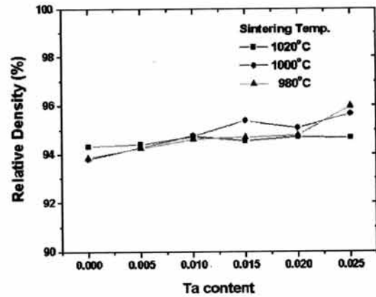
Fig. 10. Relative density of (\text{NKL})\text{N}_{1-x}\text{T}_x ( 0.000 \leq x \leq 0.025 ) sintered at various temperatures.
