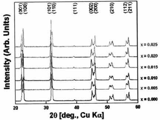
Fig. 9. XRD patterns of (\text{NKL})\text{N}_{1-x}\text{T}_x ( 0.000 \leq x \leq 0.025 ) sintered at 1,000^\circ\text{C} for 4 h.
