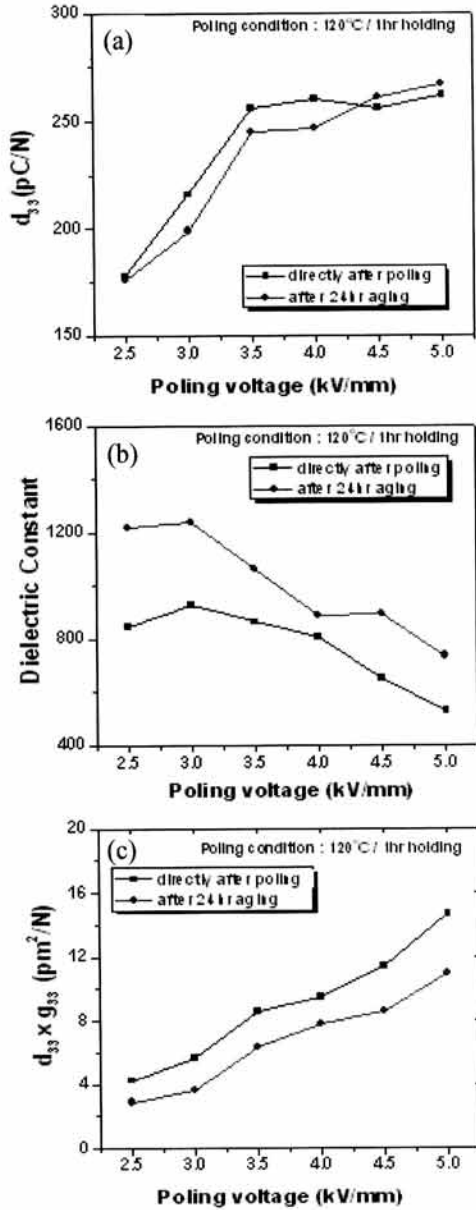
Fig. 14. (a) d_{33} , (b) \epsilon_{33}^T/\epsilon_0 and (c) d_{33} \times g_{33} of (NKN)N 0.990 T 0.010 with changing poling voltage.
