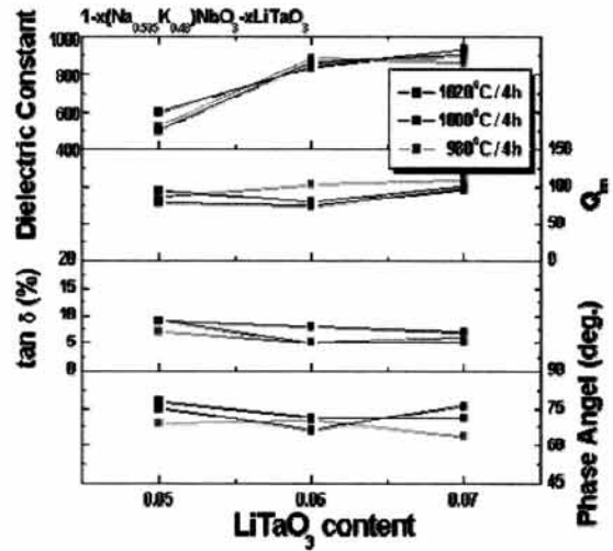
Fig. 4. \epsilon_{33}^T/\epsilon_0 , Q_m , dielectric loss ( \tan \delta ), phase angle of (1-x)NKN-xLT (0.05 ≤ x ≤ 0.07).
