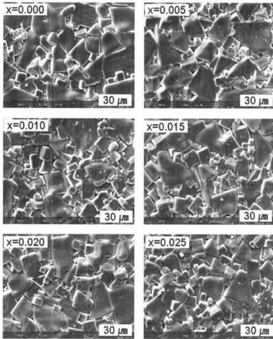
Fig. 11. SEM images of (\text{NKL})\text{N}_{1-x}\text{T}_x ( 0.000 \leq x \leq 0.025 ) sintered at various temperatures.
