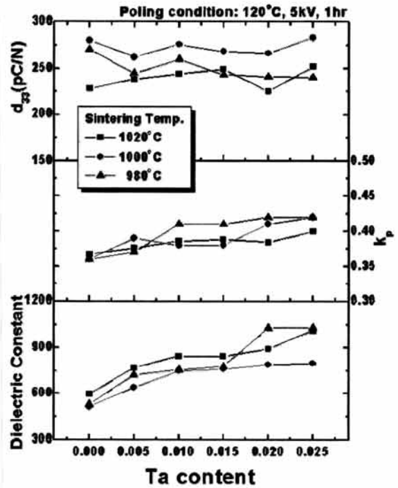
Fig. 12. d_{33} , k_p and \epsilon_{33}^T/\epsilon_0 of (\text{NKL})\text{N}_{1-x}\text{T}_x ( 0.000 \leq x \leq 0.025 ) sintered at various temperatures.
