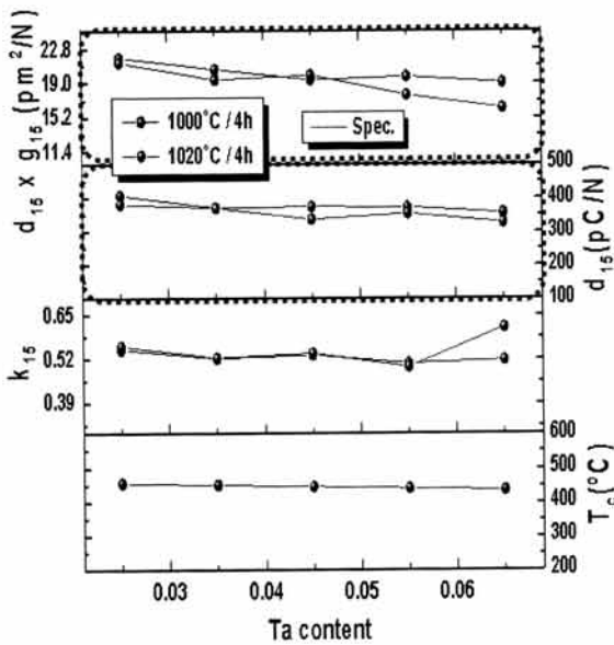
Fig. 8. d_{15} \times g_{15} , d_{15} , k_{15} and T_c of (\text{NKL})\text{N}_{1-x}\text{T}_x ( 0.025 \leq x \leq 0.065 ) sintered at various temperatures.
