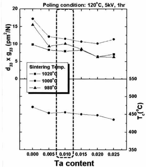
Fig. 13. d_{33} \times g_{33} and T_c of (\text{NKL})\text{N}_{1-x}\text{T}_x ( 0.000 \leq x \leq 0.025 ) sintered at various temperatures
