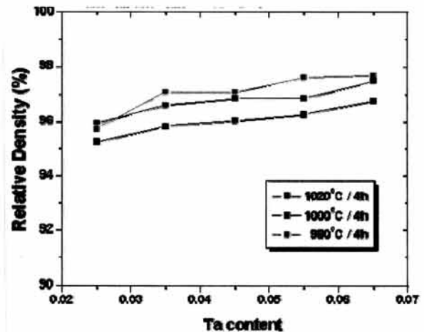
Fig. 7. Relative density of (\text{NKL})\text{N}_{1-x}\text{T}_x ( 0.025 \leq x \leq 0.065 ) sintered at various temperatures.
