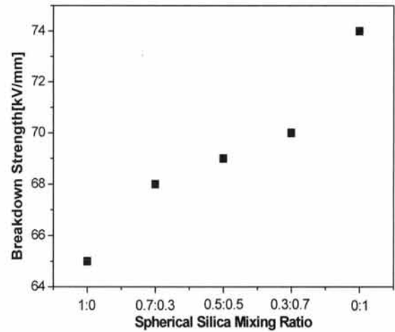
Fig. 3. Insulation breakdown strength in epoxy/spherical silica (65 wt%) systems with different mixing ratio of 5 \mu\text{m} to 20 \mu\text{m} silicas. Insulation thick was 2 mm.
