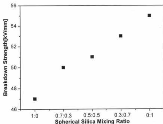
Fig. 2. Insulation breakdown strength in epoxy/spherical silica (65 wt%) systems with different mixing ratio of 5 \mu\text{m} to 20 \mu\text{m} silicas. Insulation thick was 1 mm.
