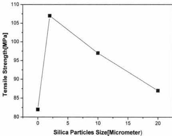
Fig. 5. Tensile strength in epoxy/silica composites (65 wt%) systems with different silica particles size (0, 2, 10, 20 \mu\text{m} ).
