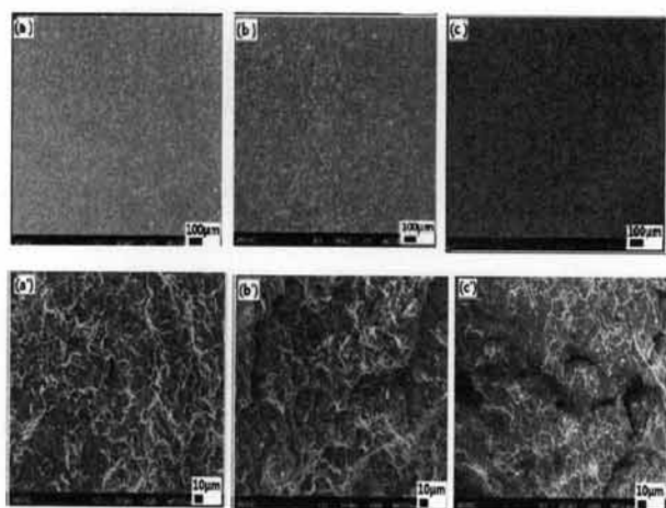
Fig. 1. FE-SEM images for epoxy/spherical silica (65 wt%) composites with various mixing ratio of 5 \mu\text{m} to 20 \mu\text{m} silicas: (a) 1 : 0 polished, (b) 0.5 : 0.5 polished, and (c) 0 : 1 polished. prime (') was done from the fractured surface after tensile test.
