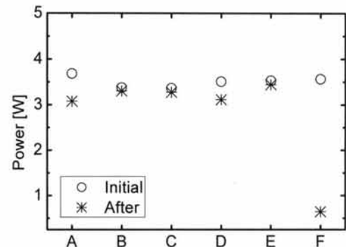
Fig. 2. Electrical power of 6 mini modules in 85°C/85% RH, -1,000 V applied to the solar cell for 3 h.
