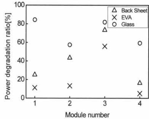
Fig. 6. Power degradation ratio of mini module biased at -1,000 V after 3 hours.
