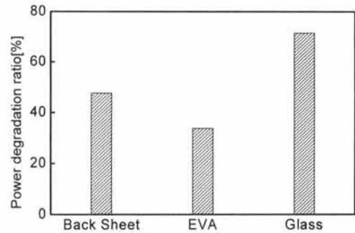
Fig. 7. Degradation ratio of average power of mini modules fabricated with various back materials after PID test.
