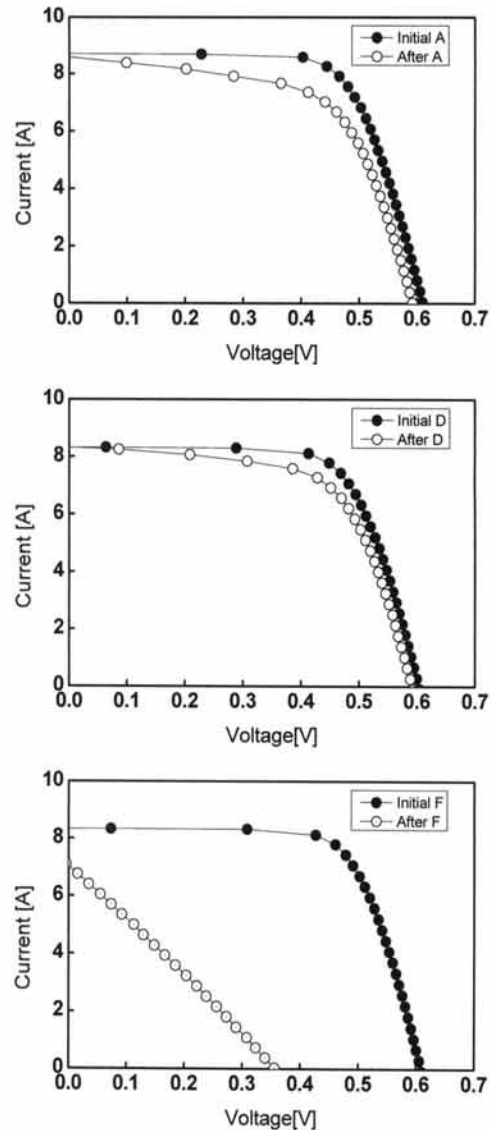
Fig. 4. Light current-voltage curve of 3 mini modules (A, D, F) by PID test.
