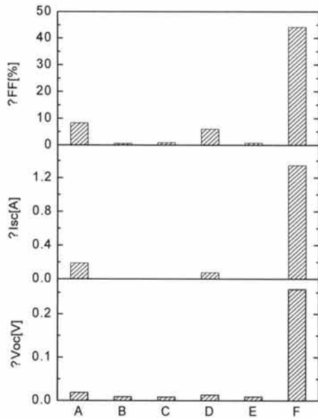
Fig. 3. Electrical characteristics of 6 mini modules in 85% RH, -1,000 V applied to the solar cell for 3 h.
