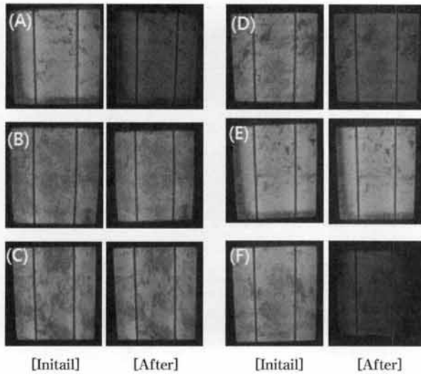
Fig. 5. Electro luminescence image of 6 mini modules before (left) and after (right) PID test.
