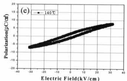
Fig. 4. P-E hysteresis loops of BCTZ ceramic as a function of different temperature. (a) 25^\circ\text{C} , (b) 50^\circ\text{C} , (c) 90^\circ\text{C} , (d) 120^\circ\text{C} , (e) 140^\circ\text{C} .
