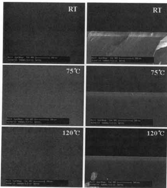
Fig. 2. SEM cross-sectional and surface images of the ITO thin films deposited on Si (001) and PET substrate at various temperatures.
