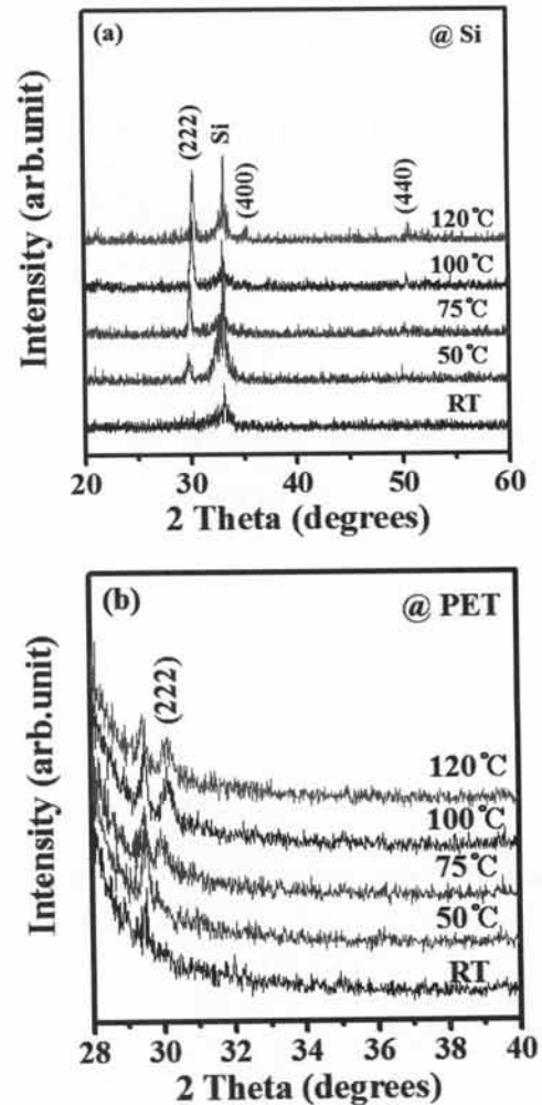
Fig. 1. XRD patterns of the ITO thin films deposited on (a) Si and (b) PET substrates at various temperatures.
