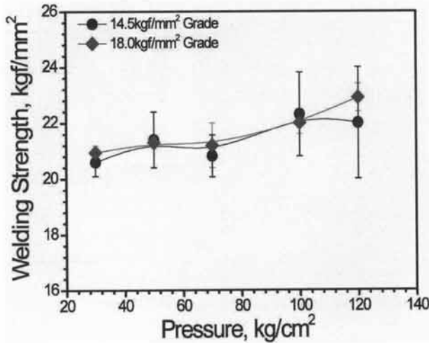
Fig. 3. Weld strength in accordance to pressure.
