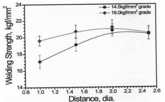
Fig. 6. Weld strength in accordance to distance at 70 kg/cm 2 pressure & 5 cycle.
