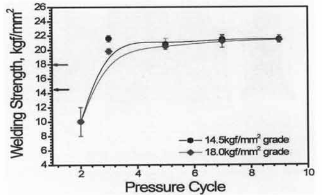
Fig. 4. Weld strength in accordance to pressure cycle at 70 kg/cm 2 pressure.
