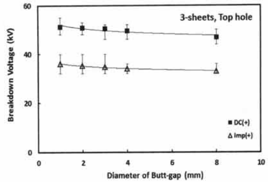
Fig. 4. Dependence of DC and impuls breakdown voltage on the diameter of butt-gap in LN 2 .
