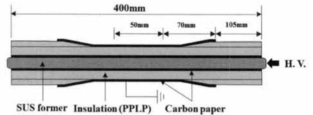
Fig. 9. Schematic diagram of mini-model cable.
