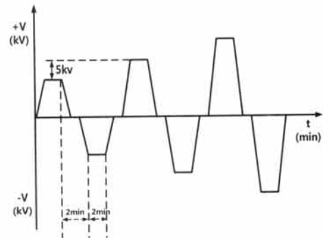
Fig. 2. DC polarity reversal profile of applied voltage.
