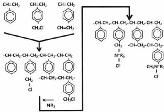
Fig. 2. Manufacture process of anion exchange membrane.
