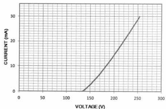
Fig. 4. Current-voltage curve of AX3220.
