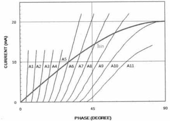
Fig. 6. Current of LED lamp as a function of phase of input voltage.
