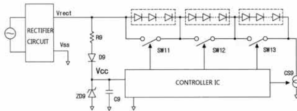
Fig. 1. Conventional LED lighting apparatus.
