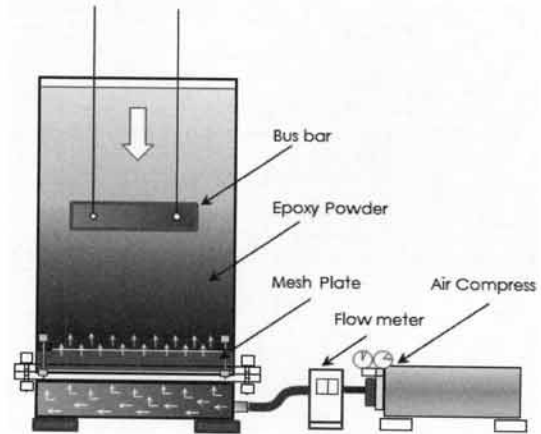
Fig. 1. Experimental setup epoxy powder coating.
