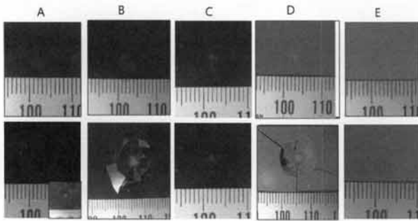
Fig. 8. Epoxy insulation of impact test.
