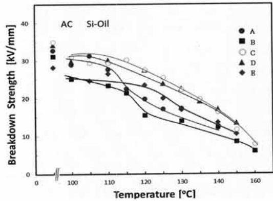
Fig. 2. AC Breakdown dependence on Temperature.
