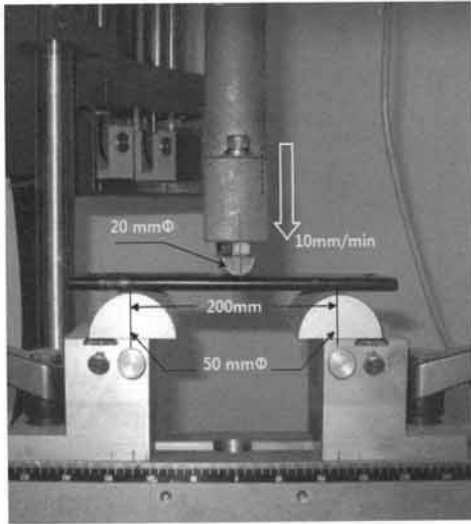
Fig. 5. Apparatus for bending test.
