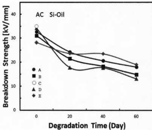
Fig. 3. AC breakdown depend on aging time.
