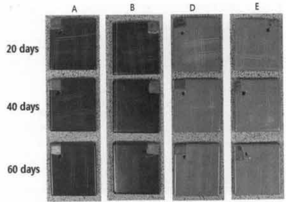
Fig. 7. Cross cut test.
