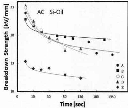
Fig. 4. V-t characteristics on degradation.
