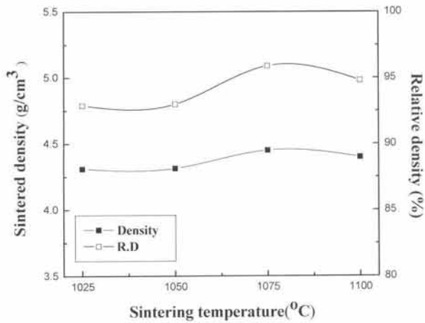
Fig. 3. Sintered density and relative density of NKN-SCT-MnO 2 specimens at varying sintering temperature.
