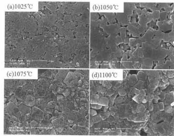
Fig. 2. Surface SEM micrographs NKN-SCT- \text{MnO}_2 specimens at varying sintering temperature: (a) 1,025^\circ\text{C} , (b) 1,050^\circ\text{C} , (c) 1,075^\circ\text{C} , and (d) 1,100^\circ\text{C} .
