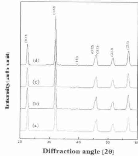
Fig. 1. XRD patterns of NKN-SCT- \text{MnO}_2 specimens as a function of sintering temperature: (a) 1,025^\circ\text{C} , (b) 1,050^\circ\text{C} , (c) 1,075^\circ\text{C} , and (d) 1,100^\circ\text{C} .
