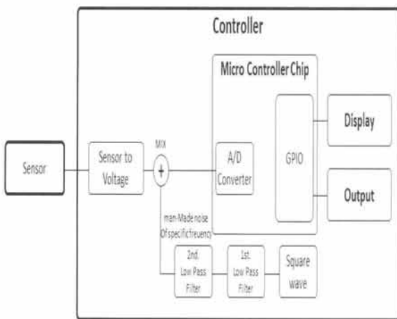
Fig. 1. Temperature control system and A/D converter concept.
