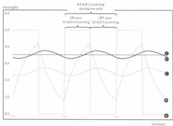
Fig. 3. Waveform of sensor signal.
